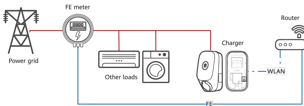
Figure 3-3 Charger connected to a router through WLAN
